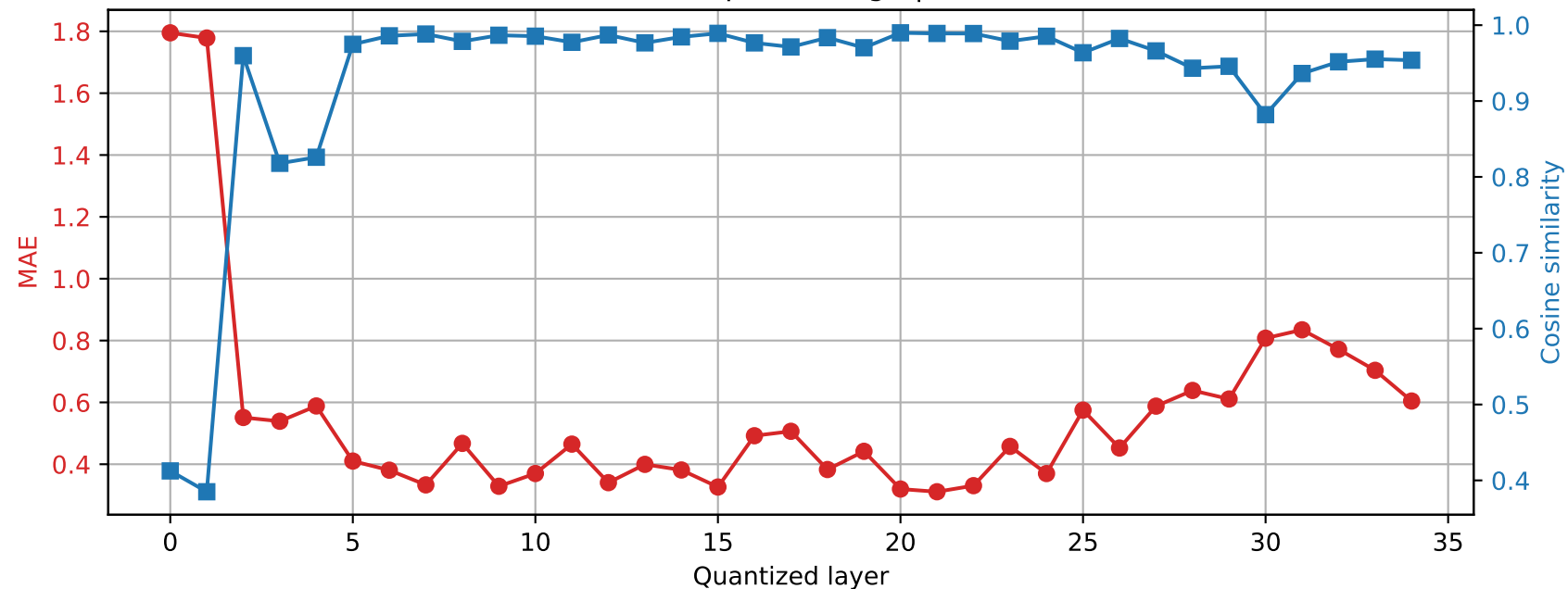
Qwen2.5-3B | Prompt 3 Final RMSNorm output damage | float32 \rightarrow int2
