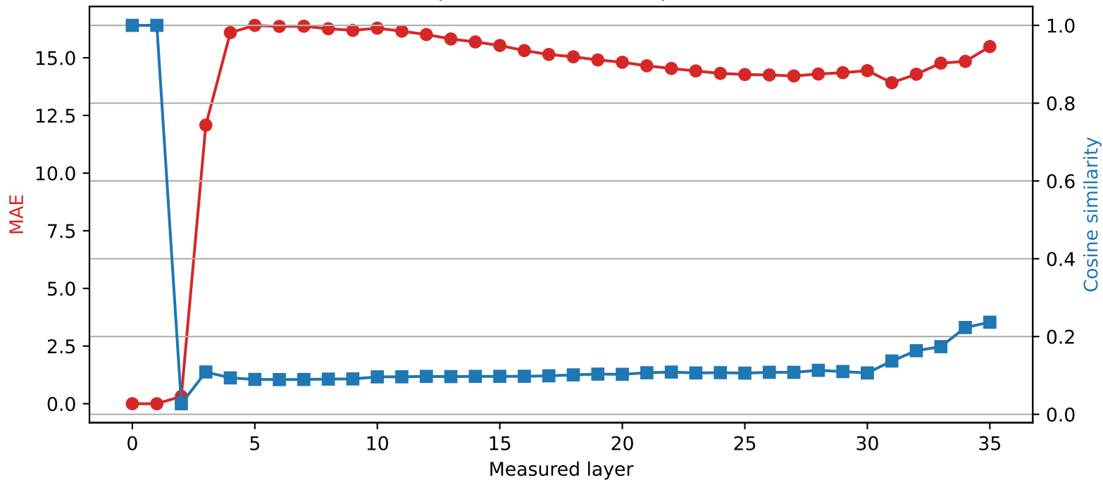
Qwen2.5-3B | Quantized layer 1 | float32 \rightarrow int2
