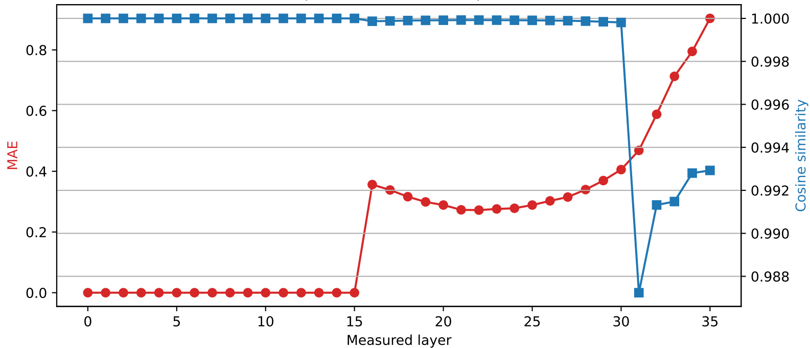
Qwen2.5-3B | Quantized layer 15 | float32 \rightarrow int2
