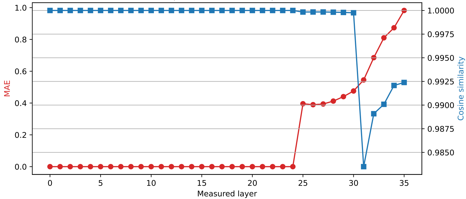
Qwen2.5-3B | Quantized layer 24 | float32 → int2
