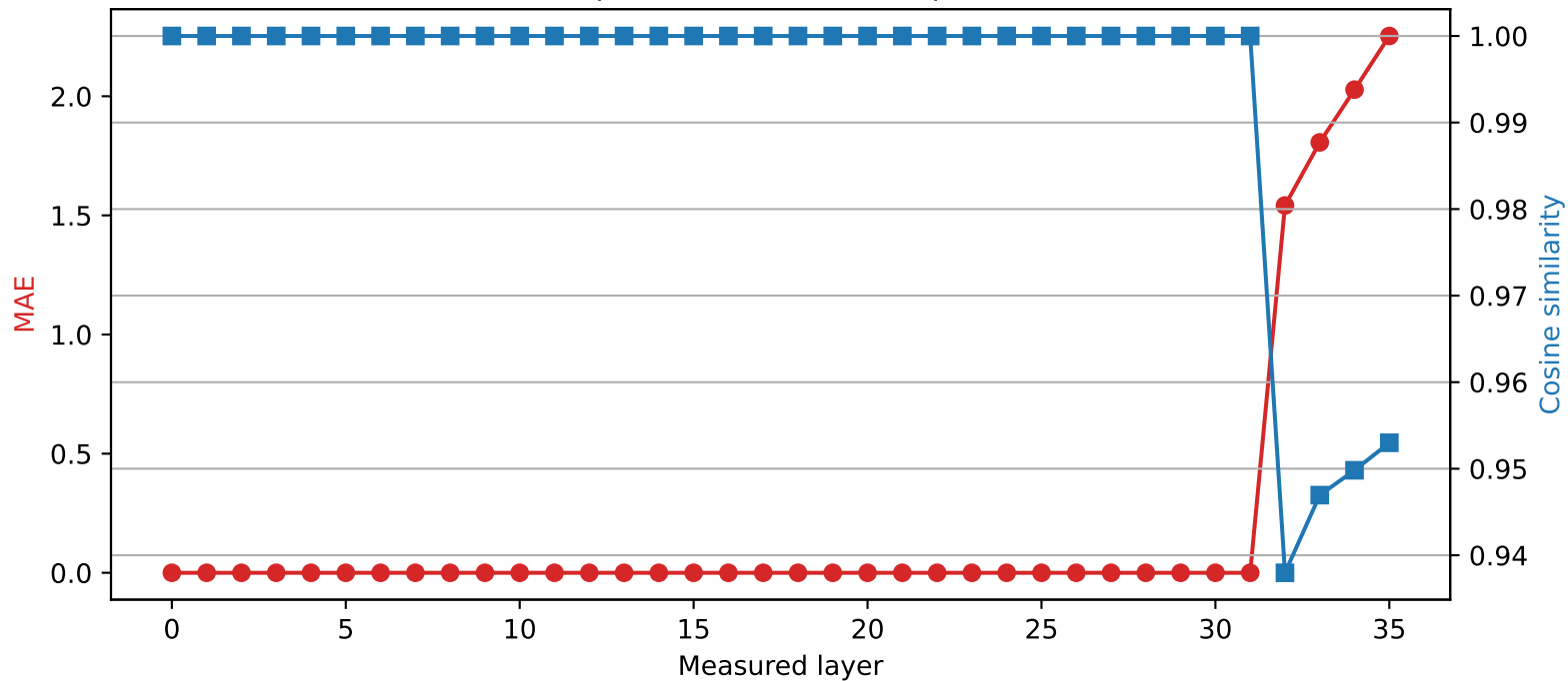
Qwen2.5-3B | Quantized layer 31 | float32 \rightarrow int2
