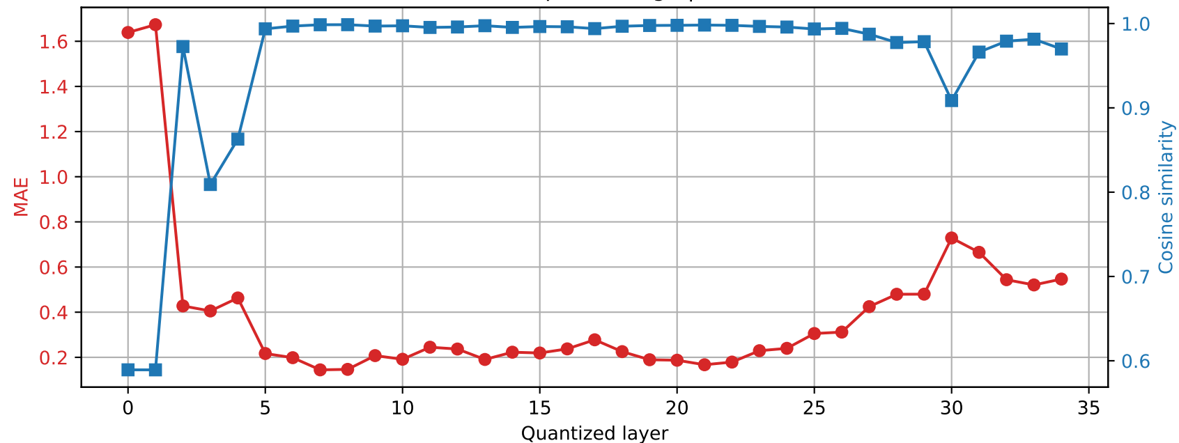
Qwen2.5-3B | Prompt 4 Final RMSNorm output damage | float32 \rightarrow int2
