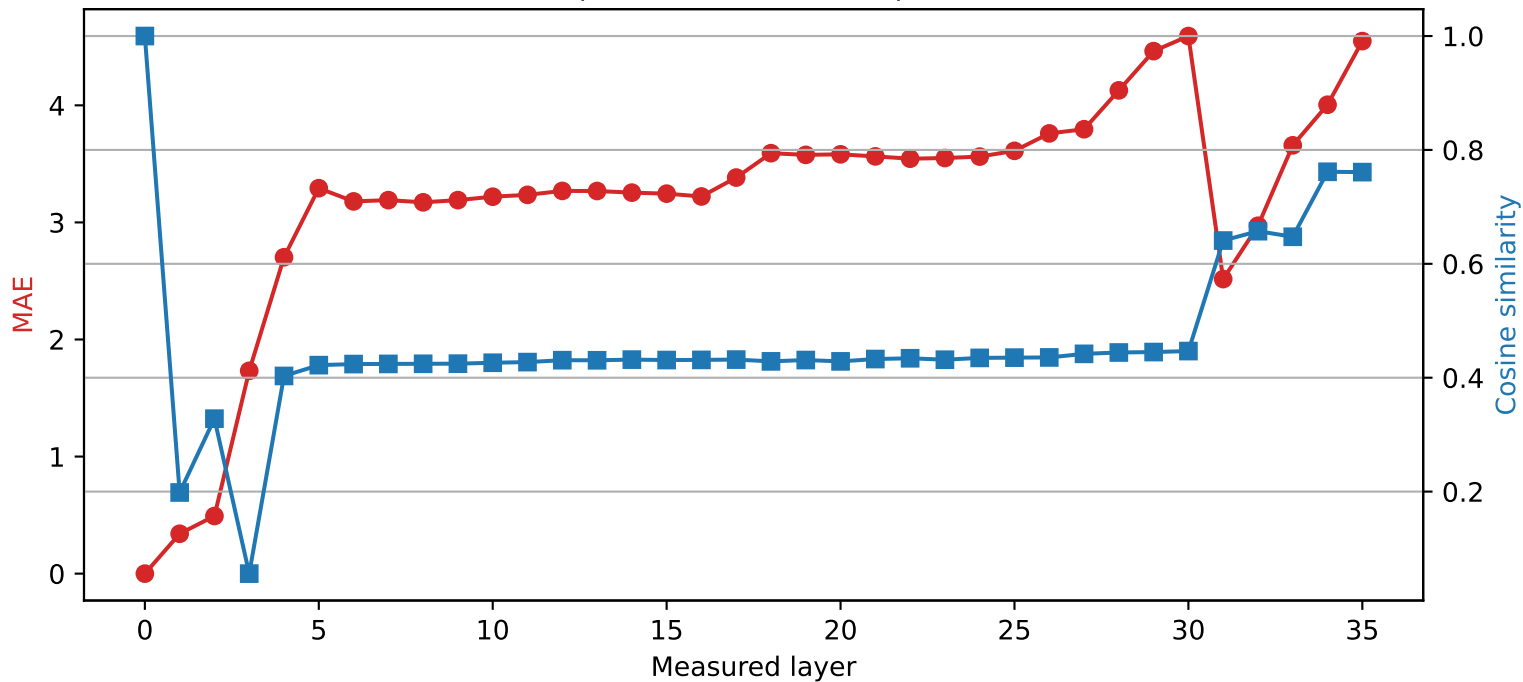
Qwen2.5-3B | Quantized layer 0 | float32 \rightarrow int2
