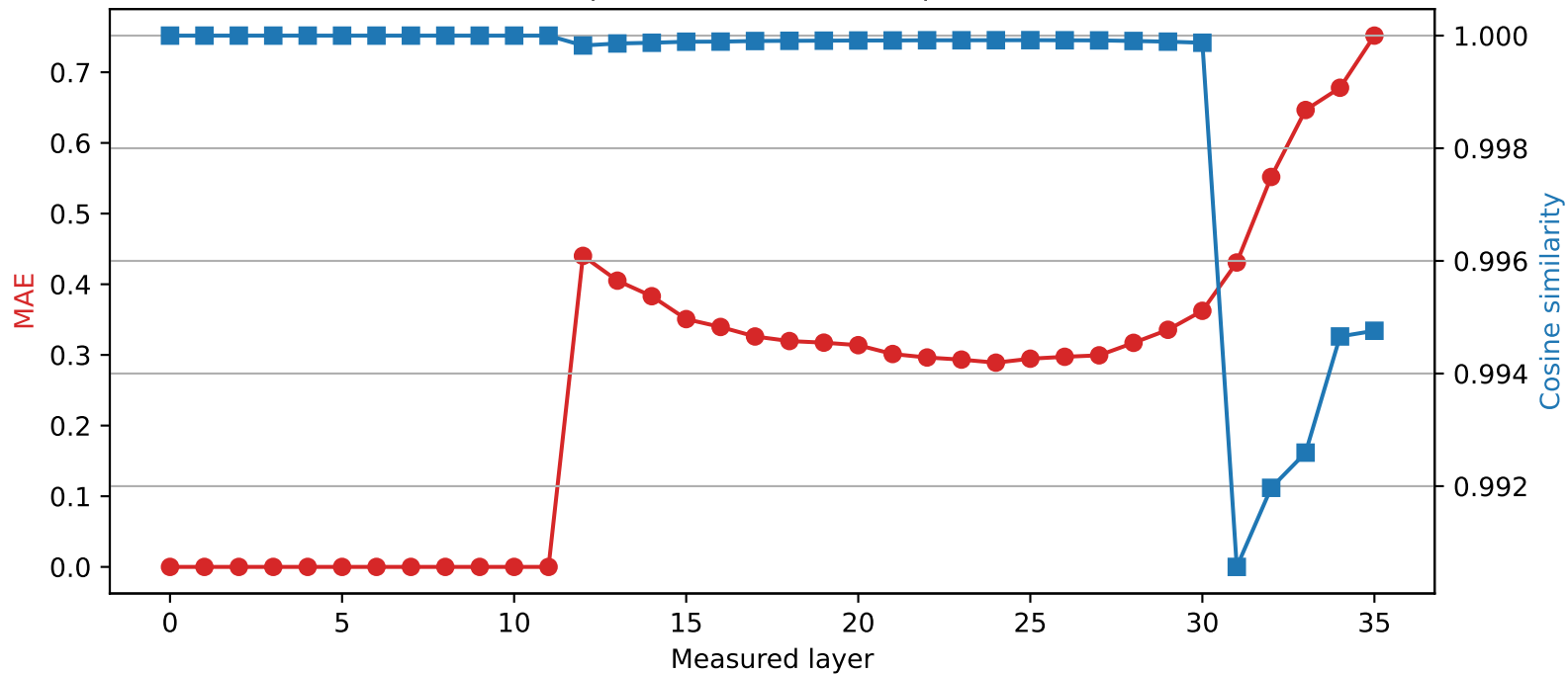
Qwen2.5-3B | Quantized layer 11 | float32 \rightarrow int2
