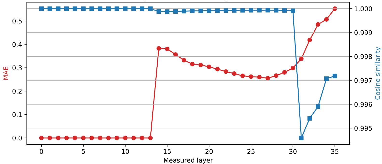
Qwen2.5-3B | Quantized layer 13 | float32 → int2
