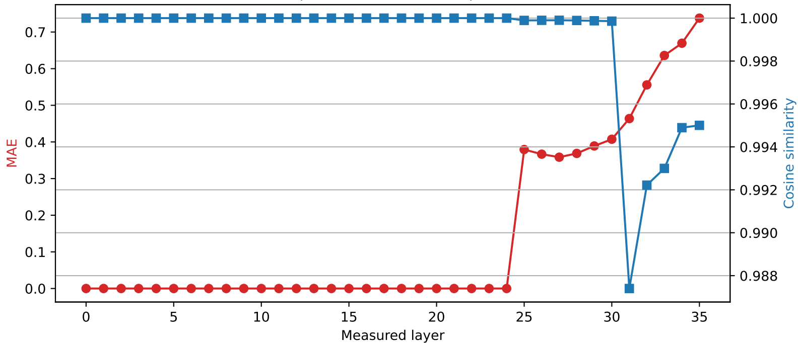
Qwen2.5-3B | Quantized layer 24 | float32 \rightarrow int2
