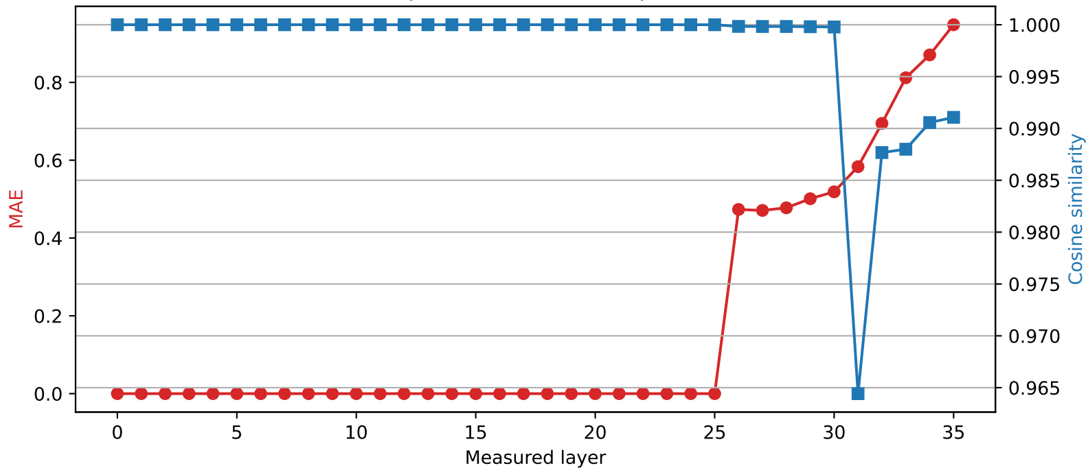
Qwen2.5-3B | Quantized layer 25 | float32 \rightarrow int2
