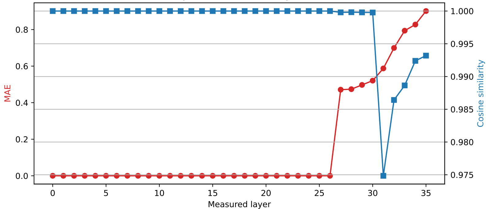
Qwen2.5-3B | Quantized layer 26 | float32 \rightarrow int2
