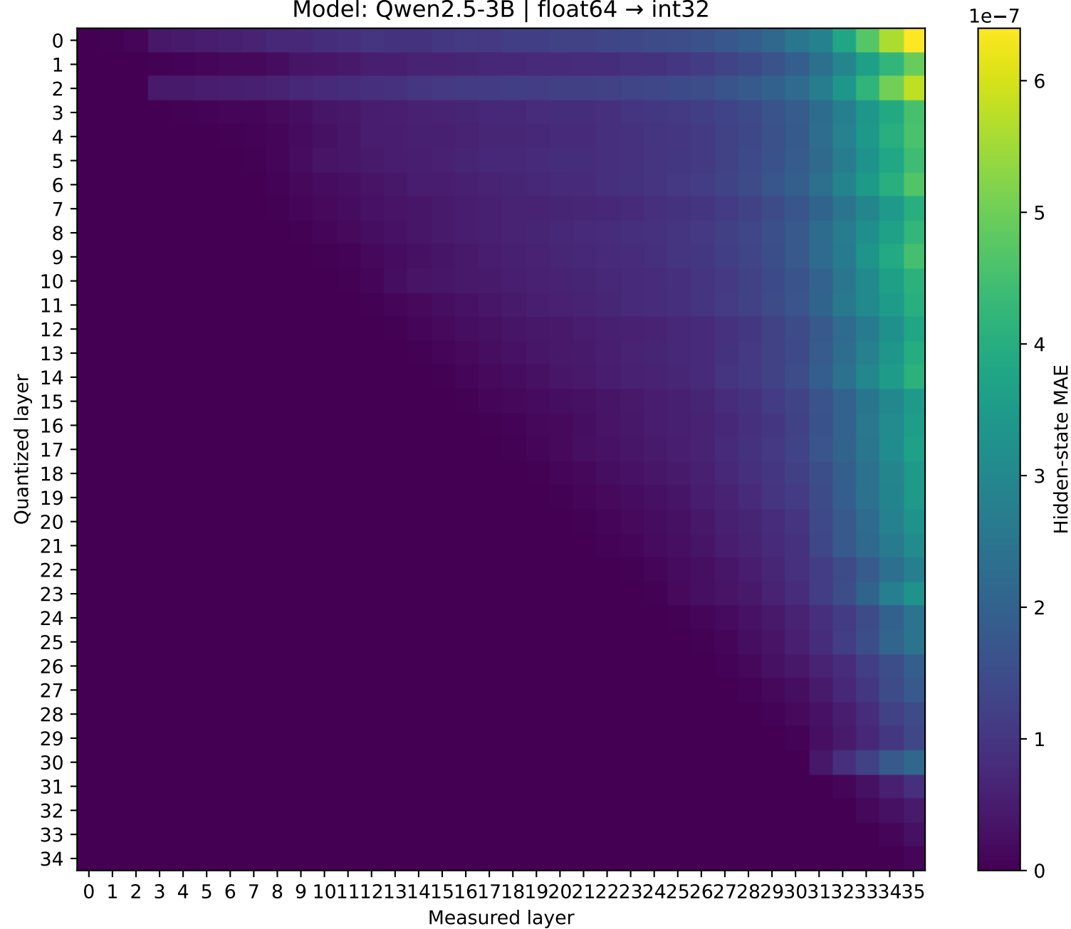
Model: Qwen2.5-3B | float64 \rightarrow int32
