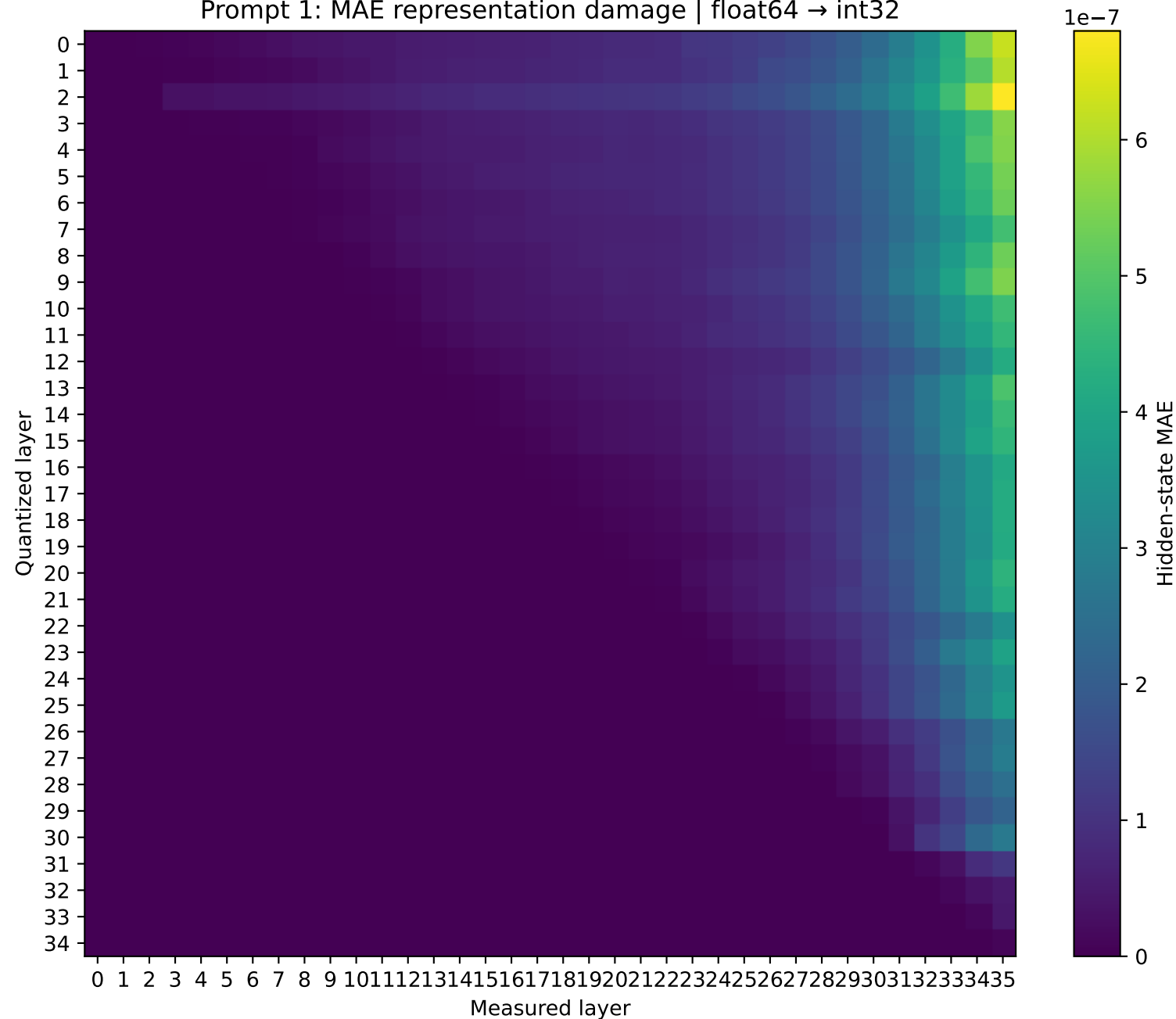
Qwen2.5-3B Prompt 1: MAE representation damage | float64 → int32
