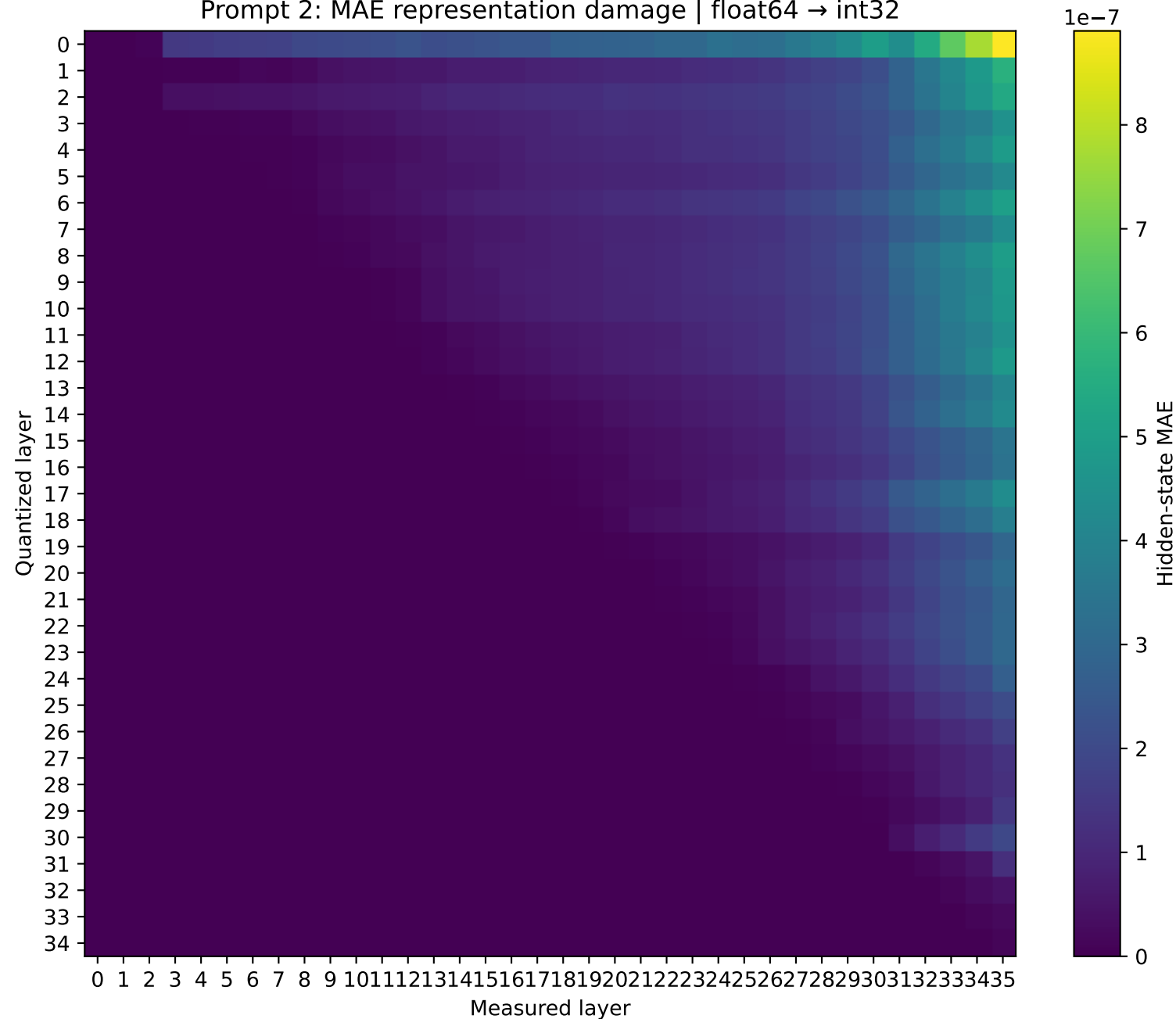
Qwen2.5-3B Prompt 2: MAE representation damage | float64 → int32
