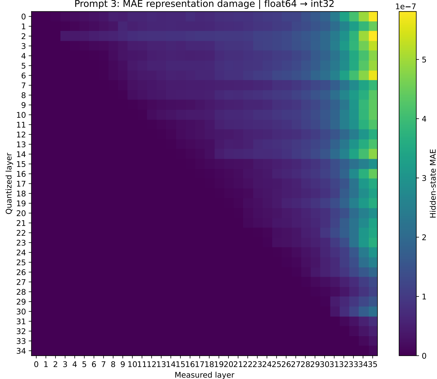
Qwen2.5-3B Prompt 3: MAE representation damage | float64 → int32
