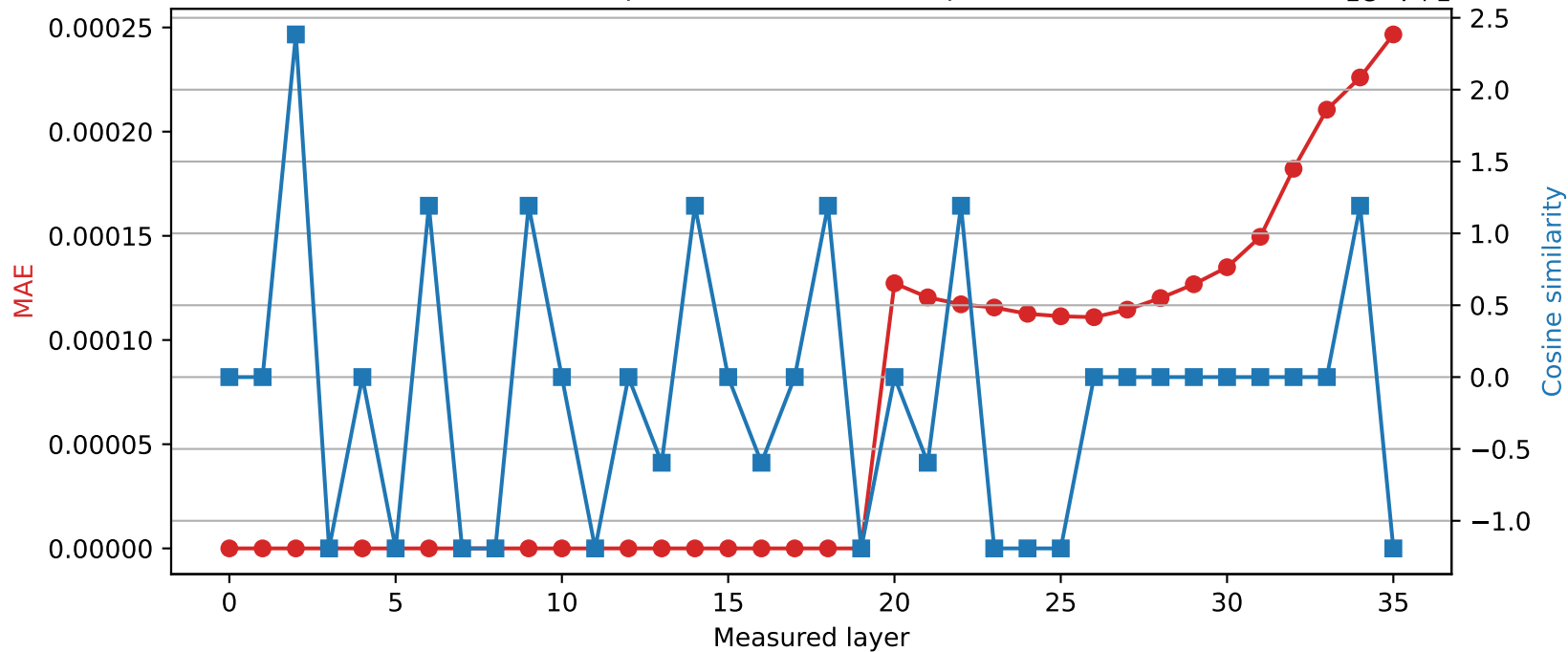
Qwen2.5-3B | Quantized layer 19 | float64 → int16
