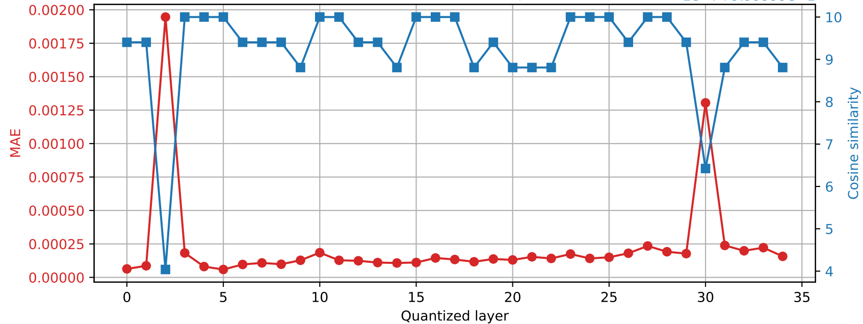
Qwen2.5-3B | Prompt 1 Final RMSNorm output damage | float64 → int16
