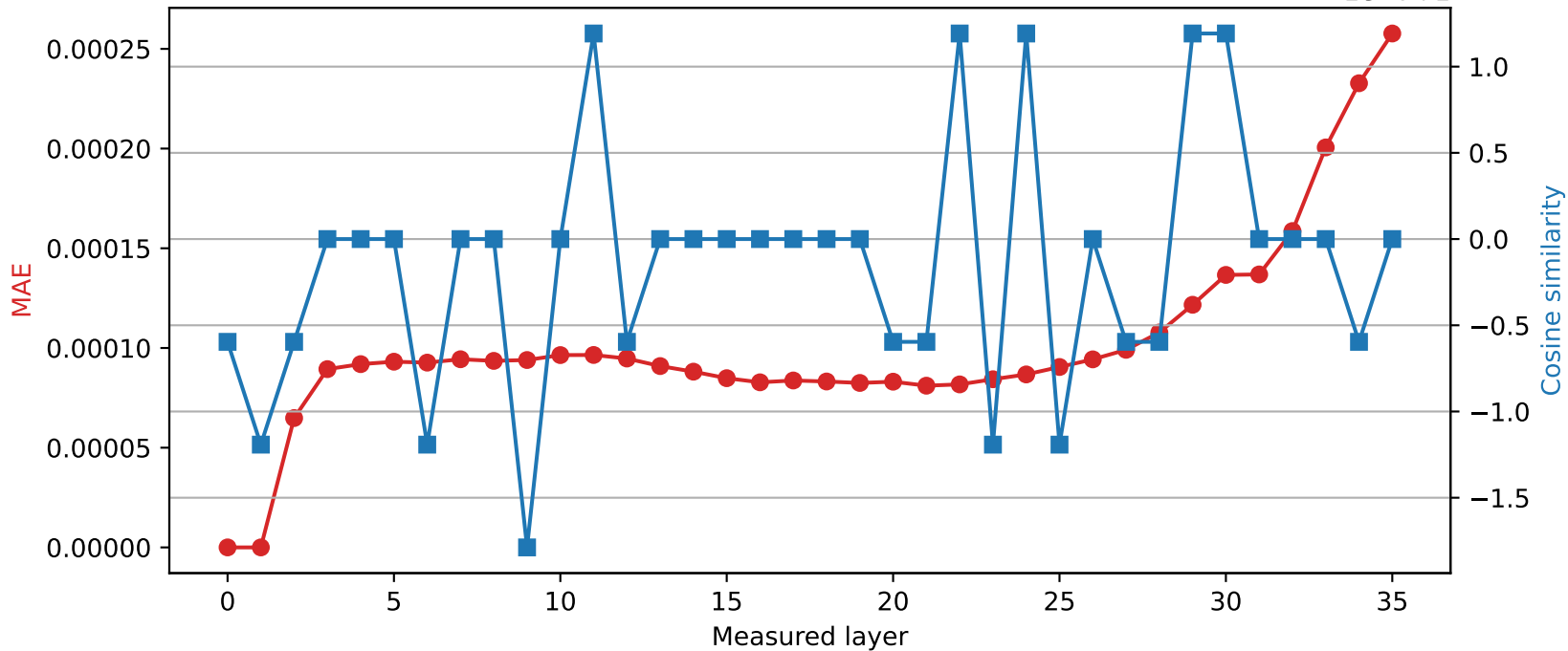
Qwen2.5-3B | Quantized layer 1 | float64 → int16
