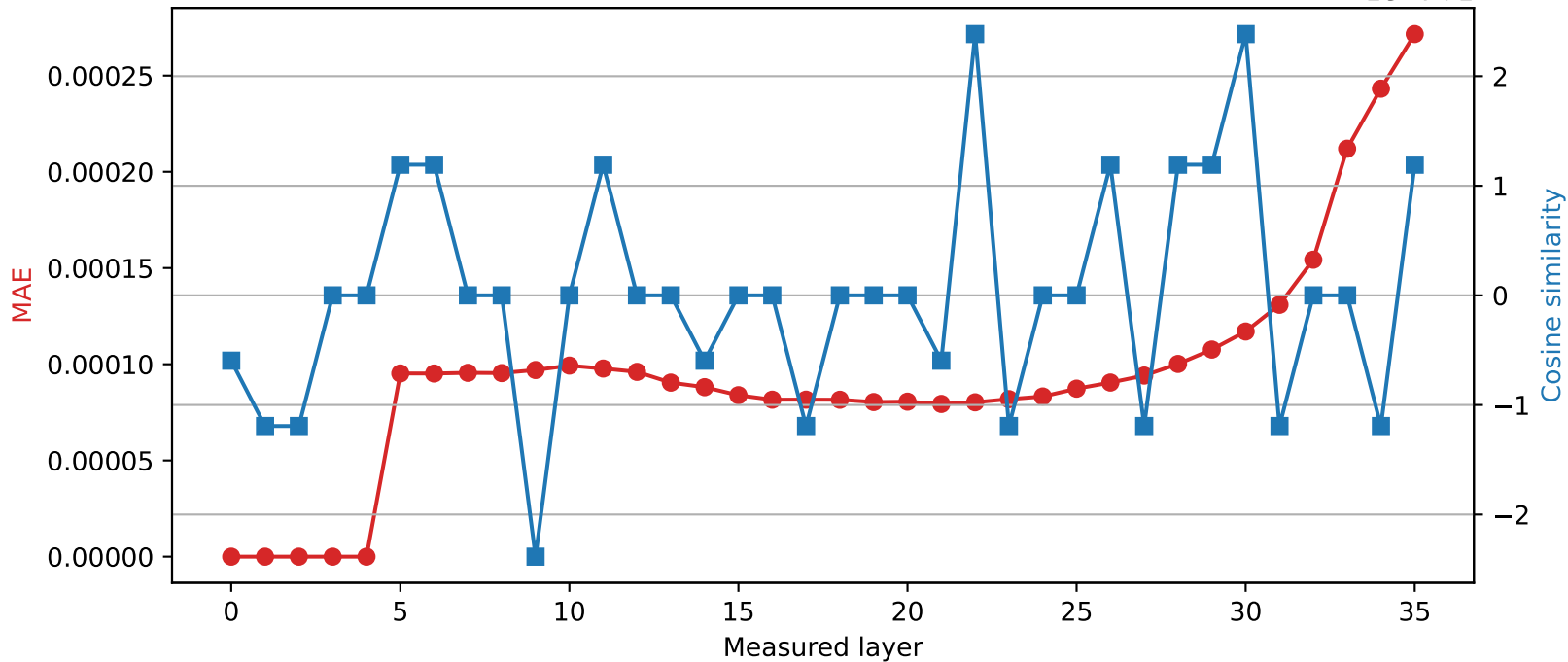
Qwen2.5-3B | Quantized layer 4 | float64 → int16
