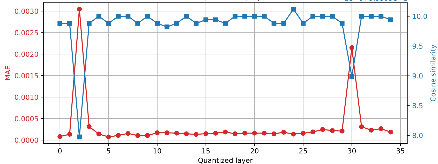
Qwen2.5-3B | Prompt 2 Final RMSNorm output damage | float64 → int16
