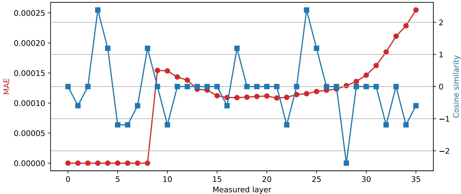
Qwen2.5-3B | Quantized layer 8 | float64 → int16
