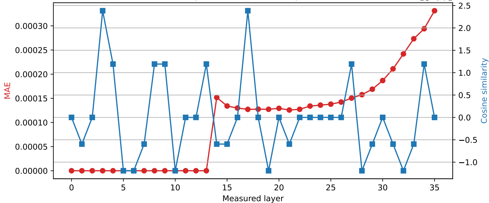
Qwen2.5-3B | Quantized layer 13 | float64 \rightarrow int16
