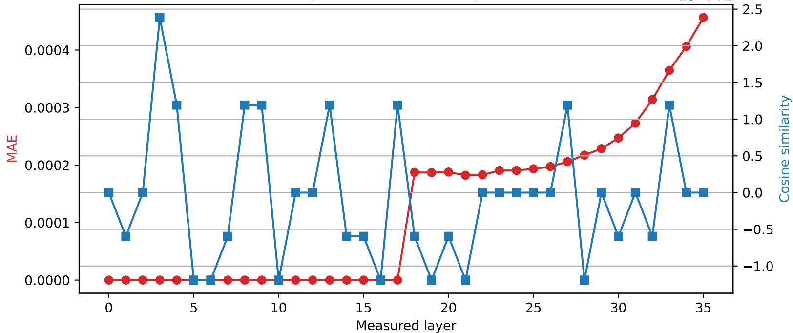
Qwen2.5-3B | Quantized layer 17 | float64 → int16
