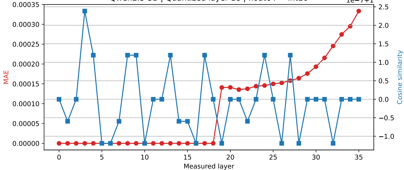
Qwen2.5-3B | Quantized layer 18 | float64 → int16
