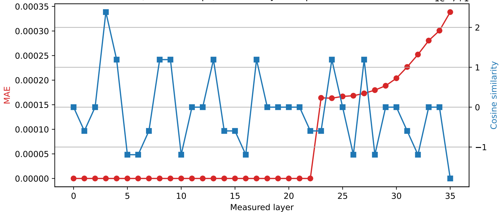
Qwen2.5-3B | Quantized layer 22 | float64 → int16
