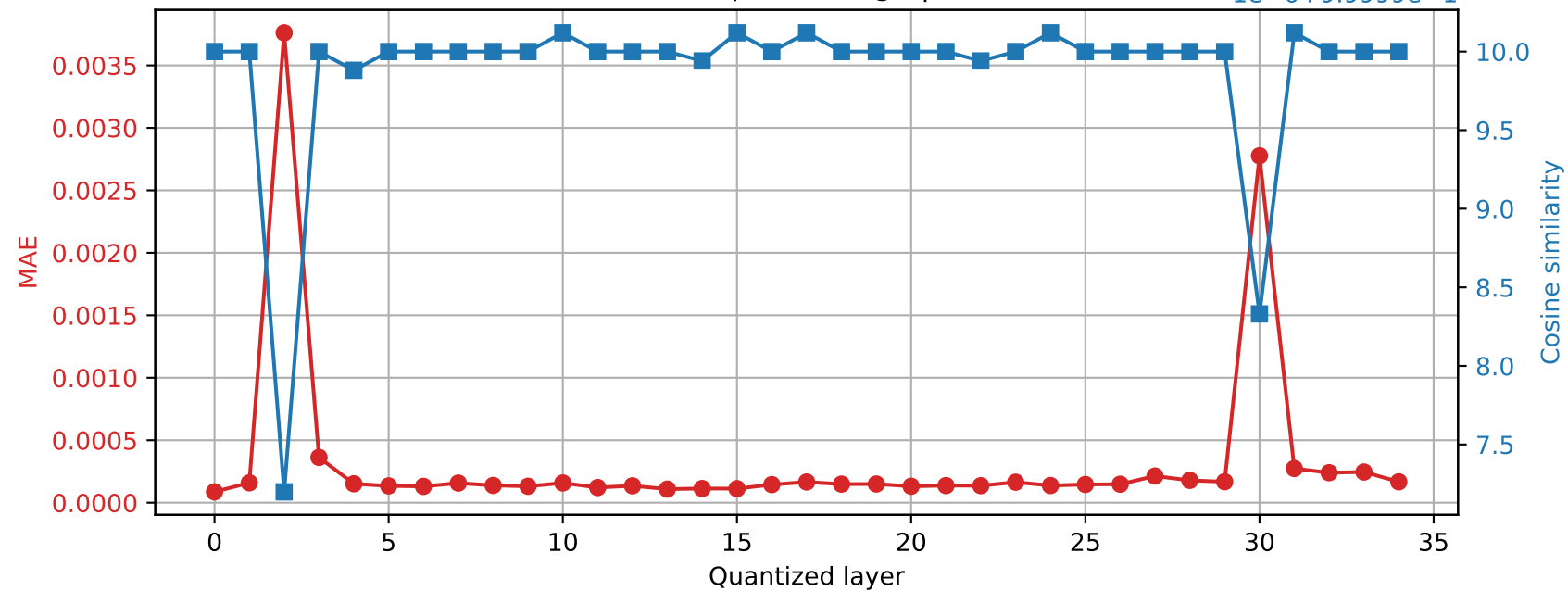
Qwen2.5-3B | Prompt 3 Final RMSNorm output damage | float64 → int16
