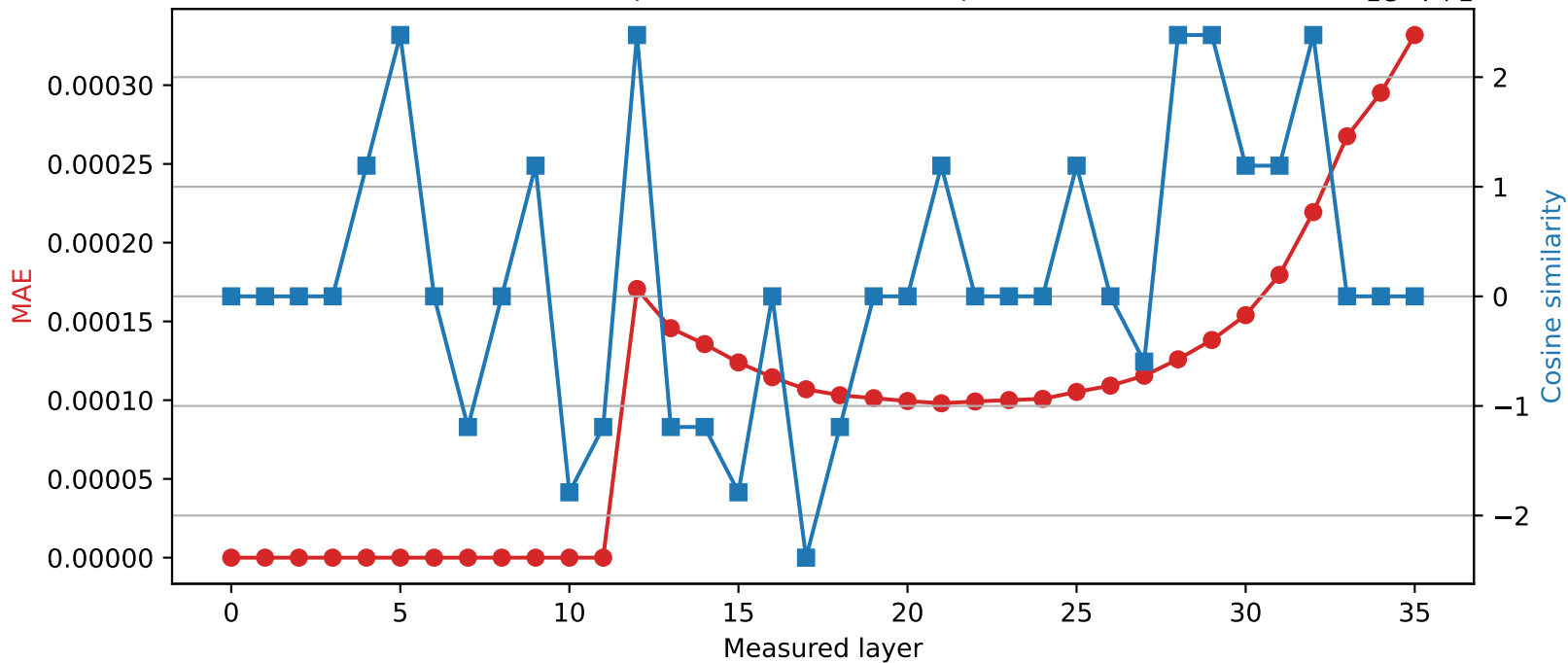
Qwen2.5-3B | Quantized layer 11 | float64 → int16
