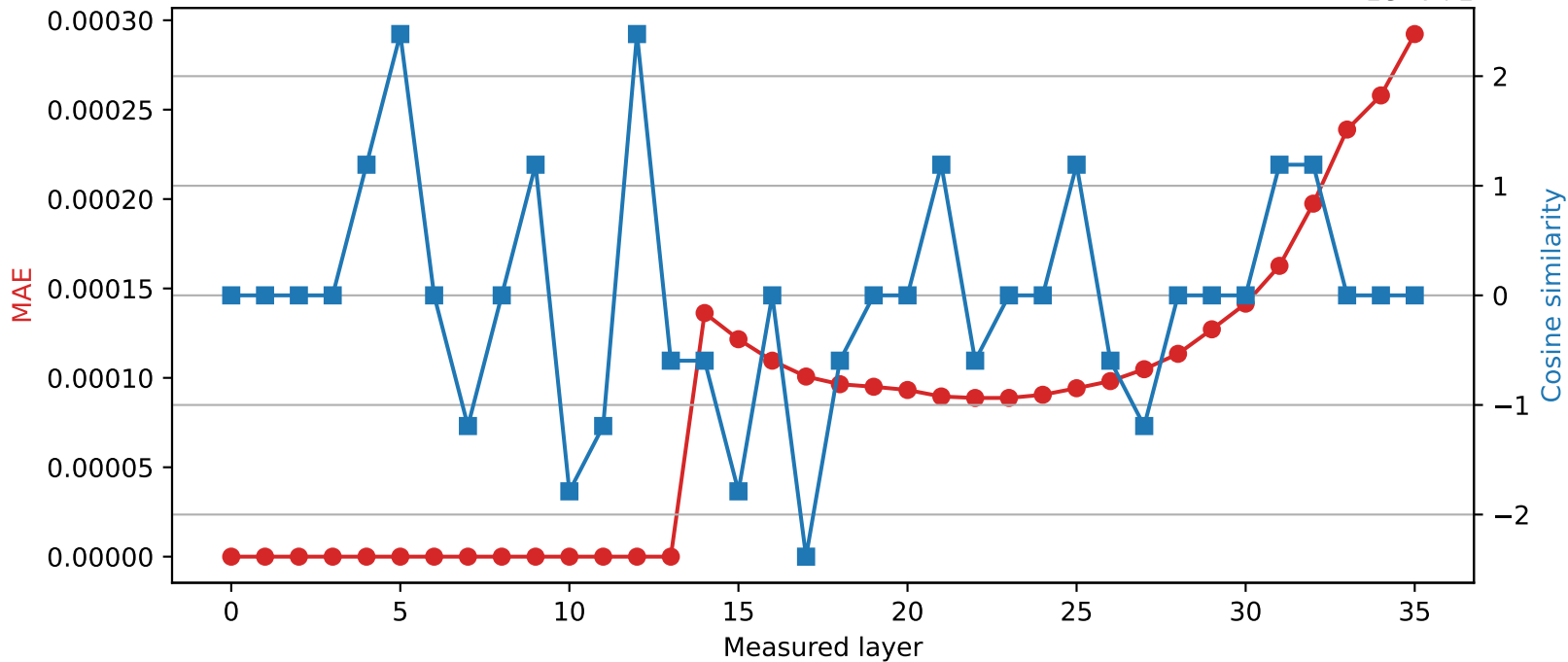
Qwen2.5-3B | Quantized layer 13 | float64 → int16
