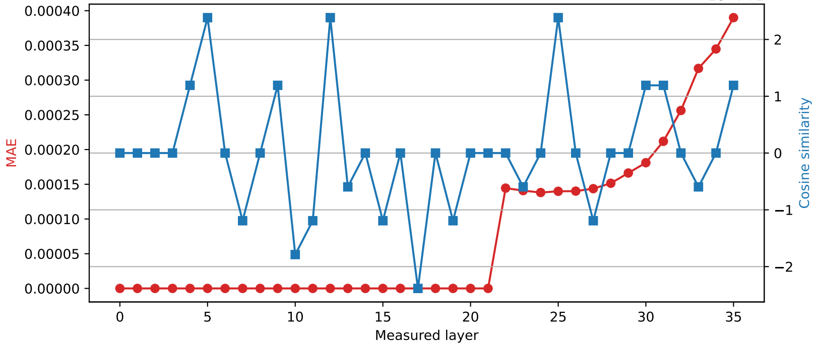
Qwen2.5-3B | Quantized layer 21 | float64 → int16
