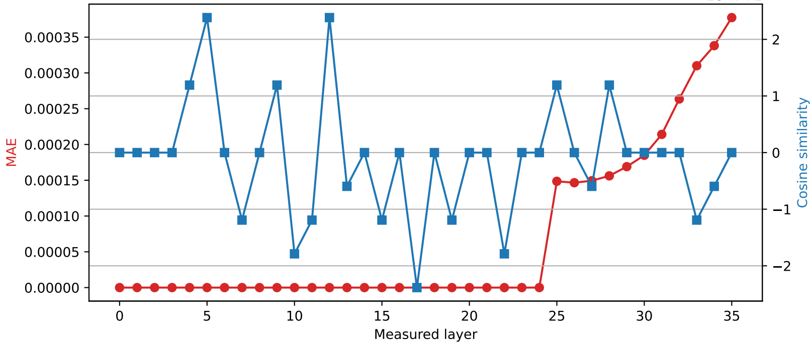
Qwen2.5-3B | Quantized layer 24 | float64 → int16
