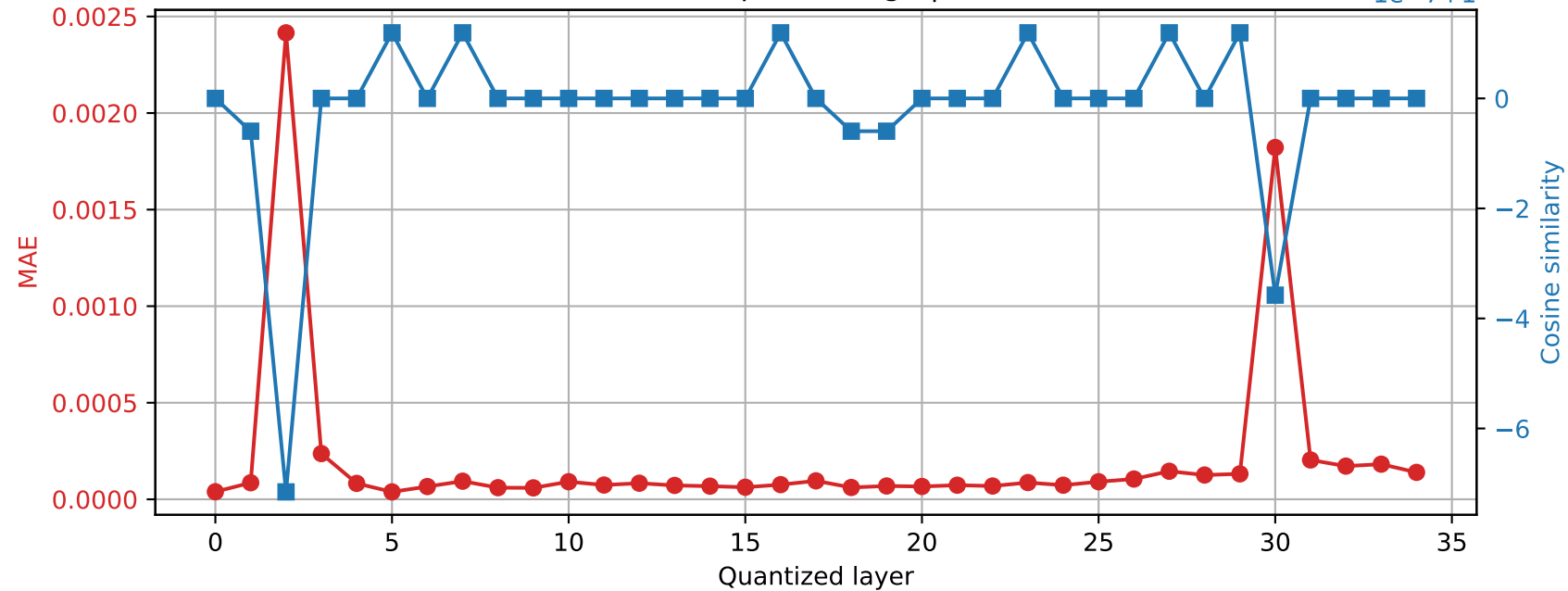
Qwen2.5-3B | Prompt 4 Final RMSNorm output damage | float64 → int16
