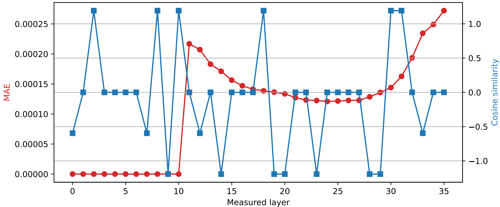
Qwen2.5-3B | Quantized layer 10 | float64 \rightarrow int16
