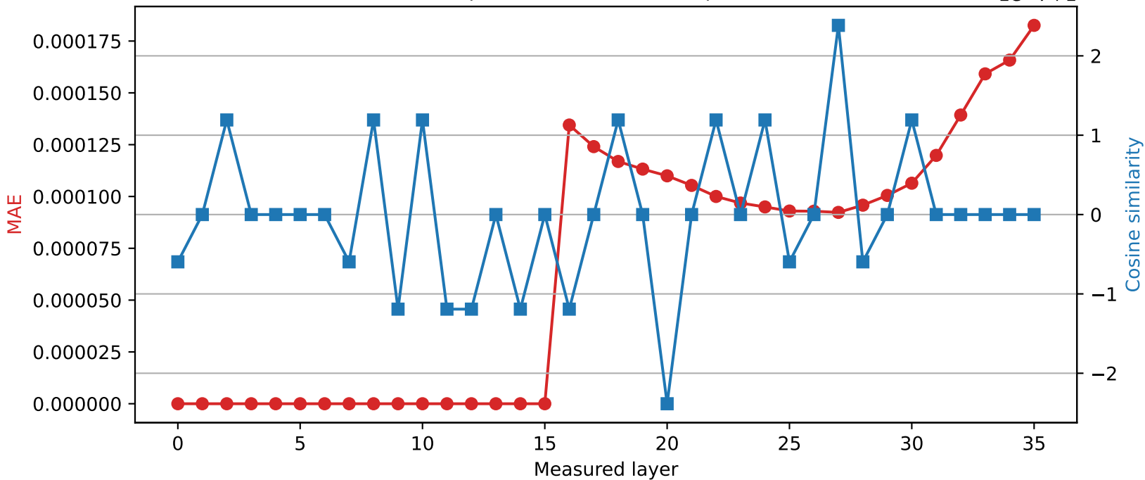
Qwen2.5-3B | Quantized layer 15 | float64 → int16
