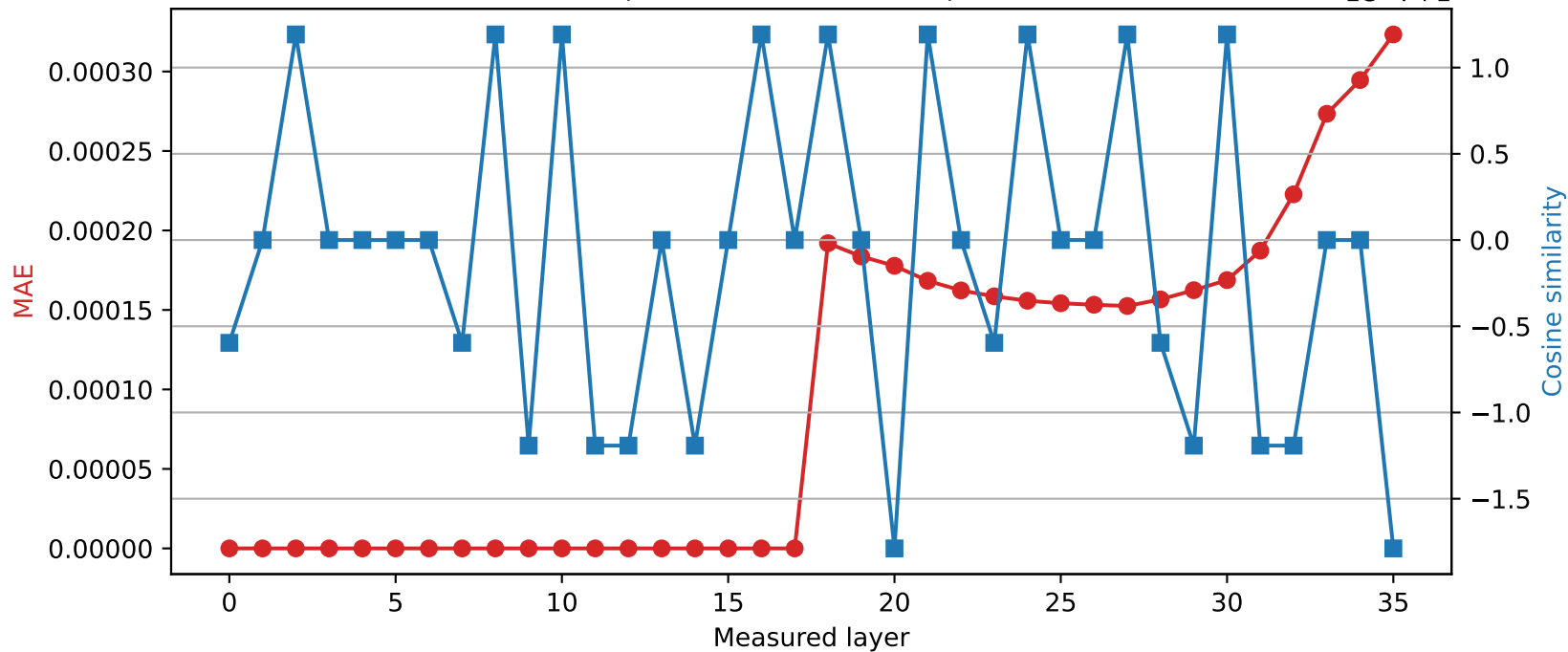
Qwen2.5-3B | Quantized layer 17 | float64 \rightarrow int16
