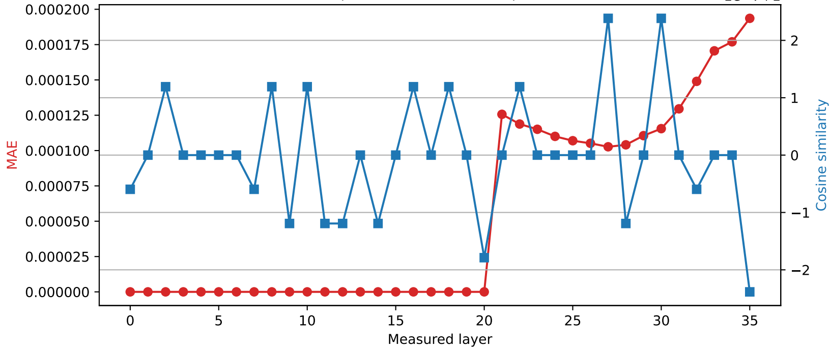
Qwen2.5-3B | Quantized layer 20 | float64 → int16
