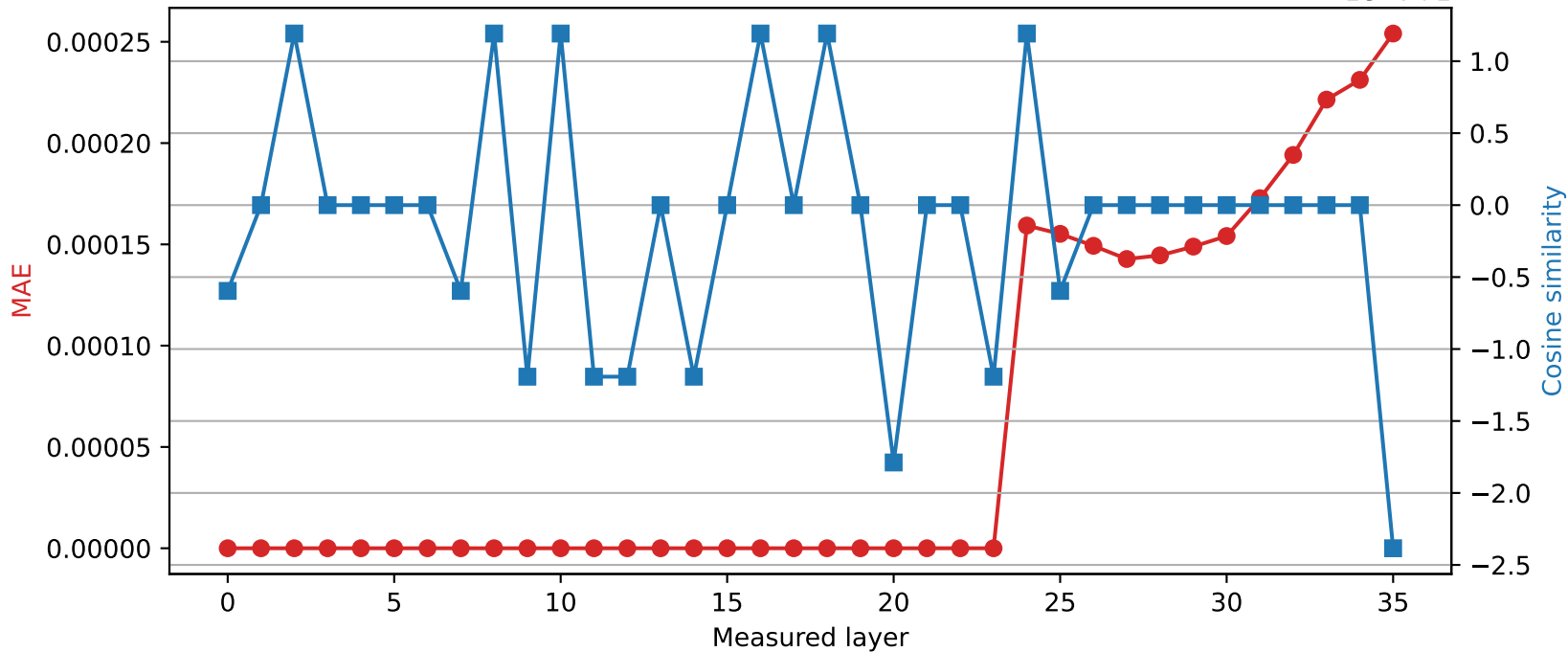
Qwen2.5-3B | Quantized layer 23 | float64 → int16
