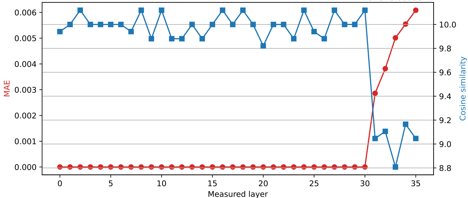
Qwen2.5-3B | Quantized layer 30 | float64 \rightarrow int16 1e-6+9.9999e-1
