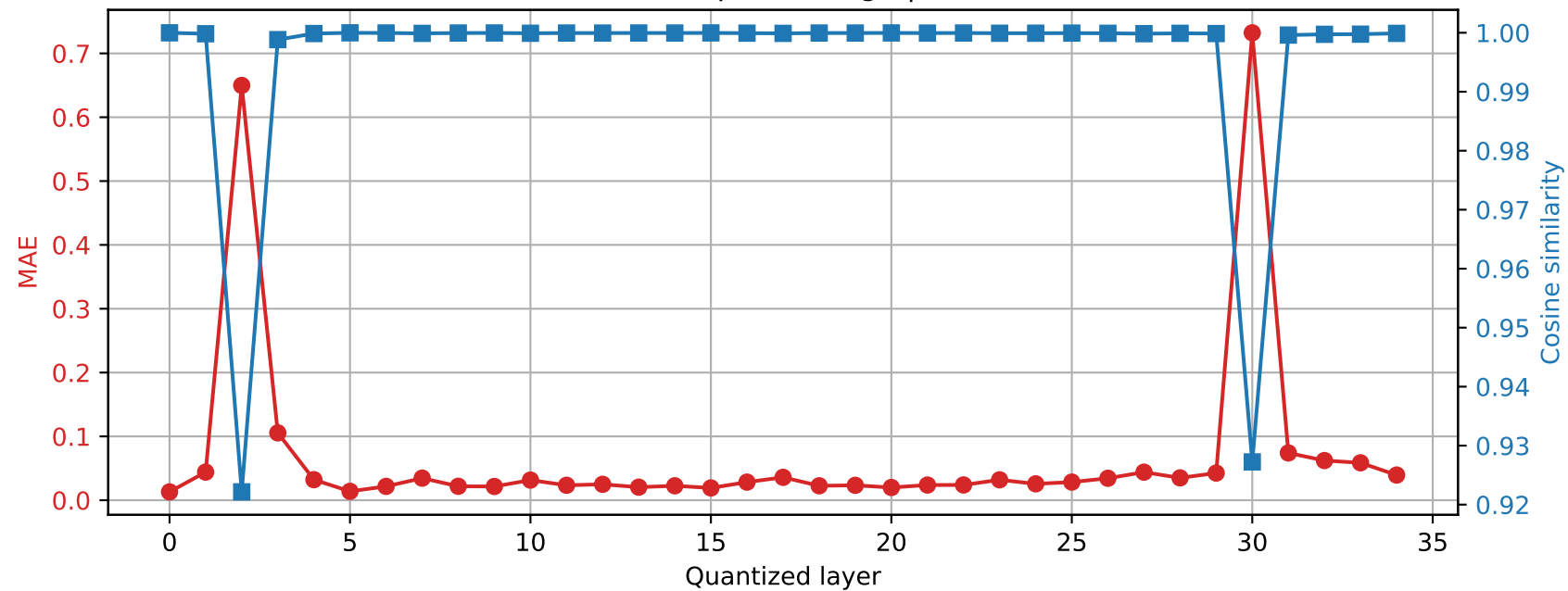
Qwen2.5-3B | Prompt 0 Final RMSNorm output damage | float64 → int8
