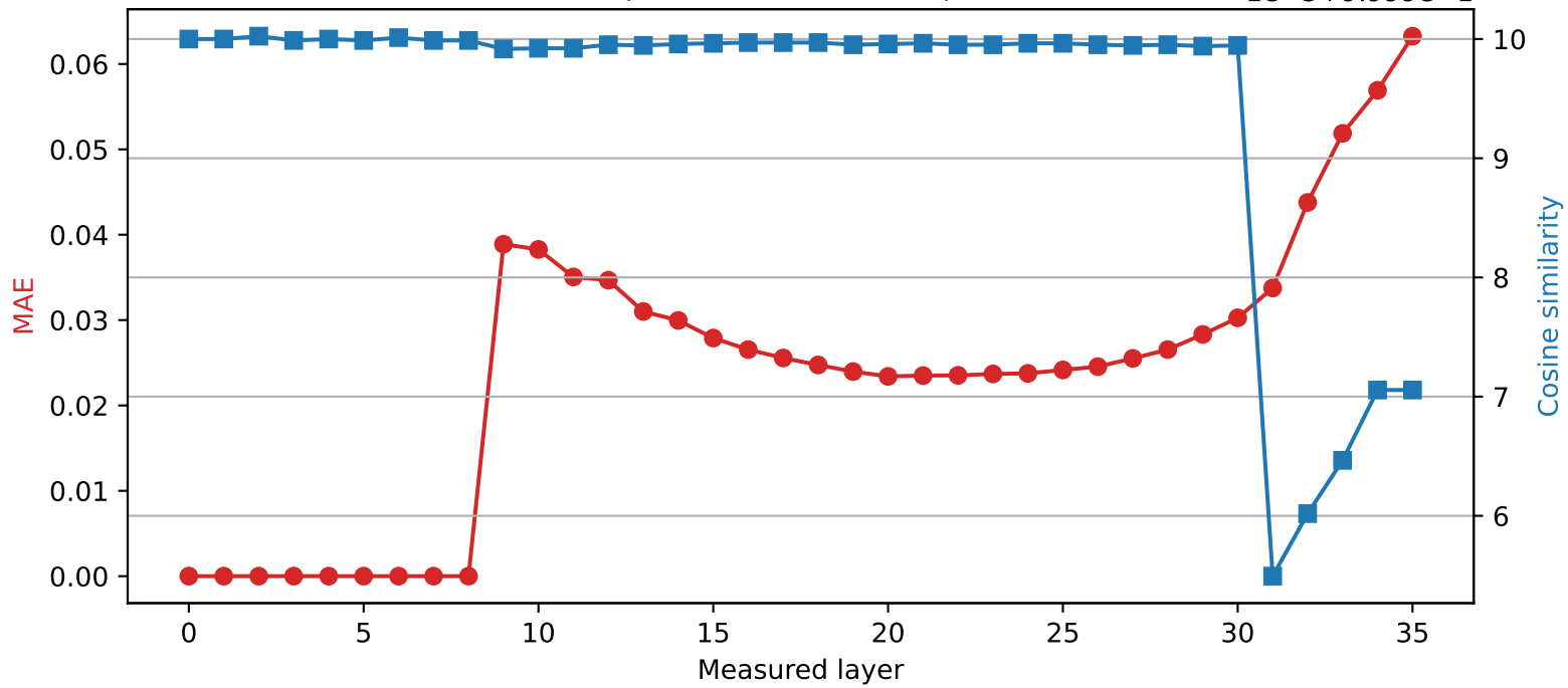
Qwen2.5-3B | Quantized layer 8 | float64 → int8
