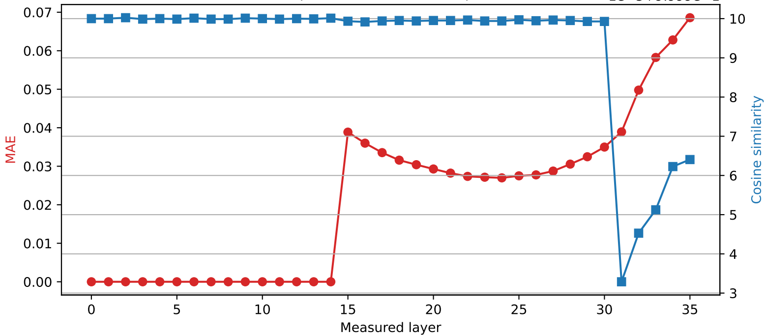
Qwen2.5-3B | Quantized layer 14 | float64 → int8
