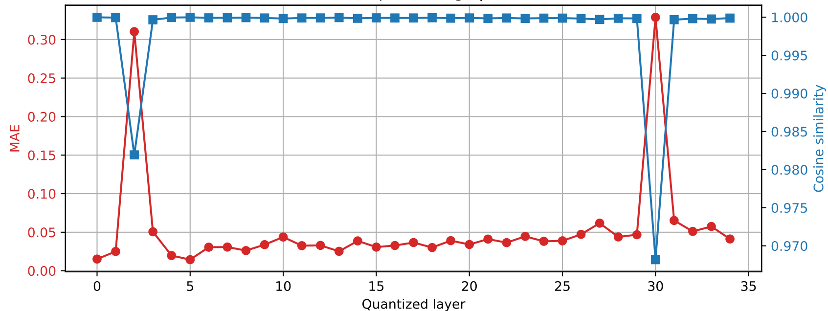
Qwen2.5-3B | Prompt 1 Final RMSNorm output damage | float64 → int8
