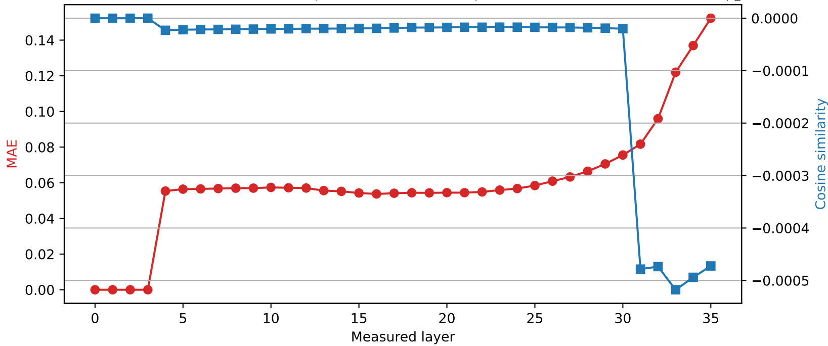
Qwen2.5-3B | Quantized layer 3 | float64 → int8
