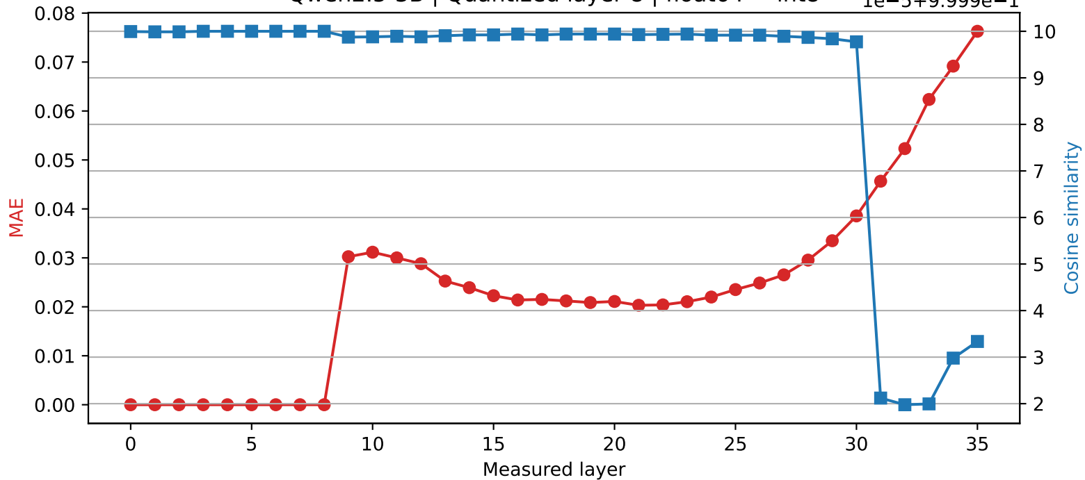
Qwen2.5-3B | Quantized layer 8 | float64 → int8
