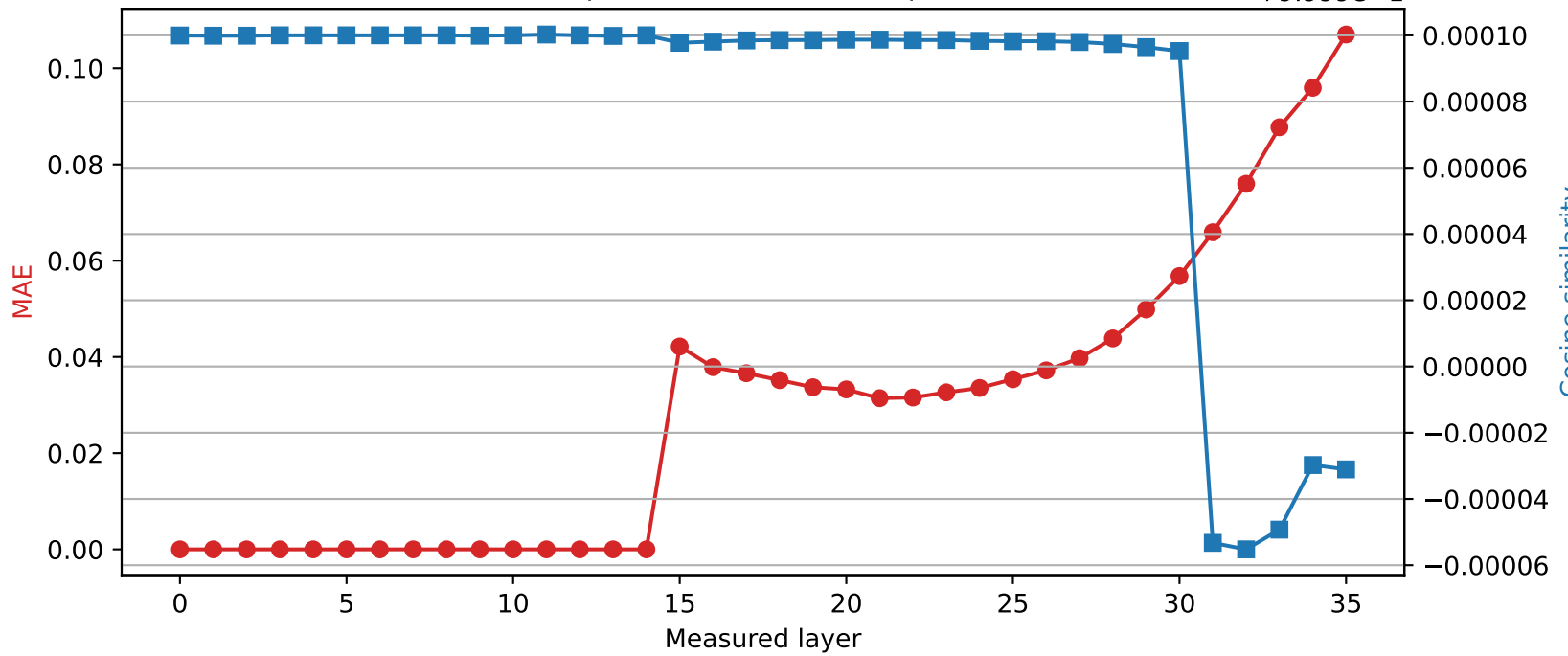
Qwen2.5-3B | Quantized layer 14 | float64 → int8
