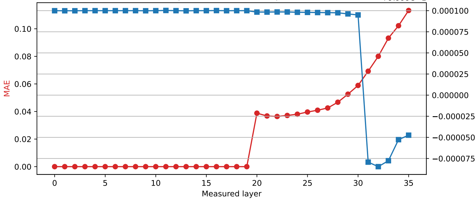
Qwen2.5-3B | Quantized layer 19 | float64 → int8
