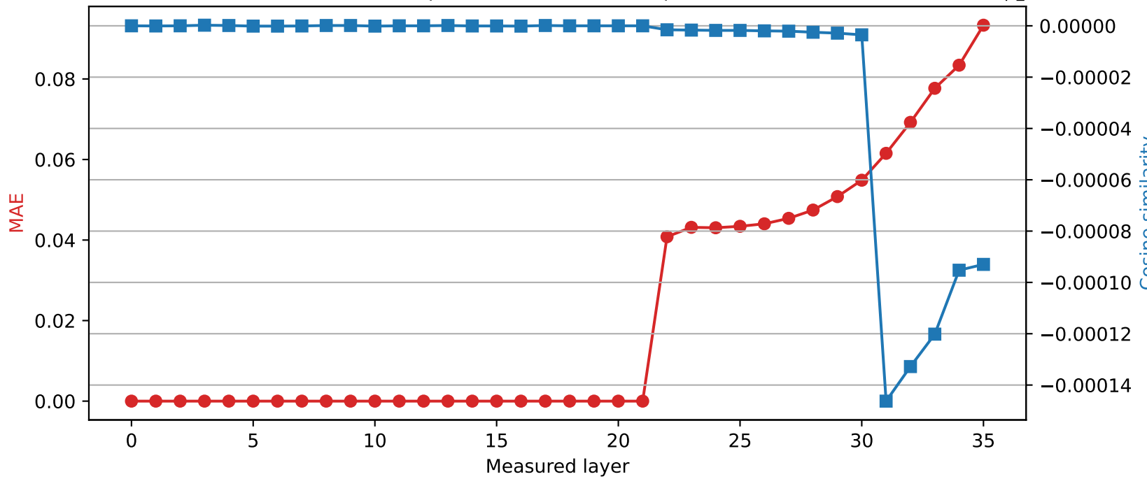
Qwen2.5-3B | Quantized layer 21 | float64 → int8
