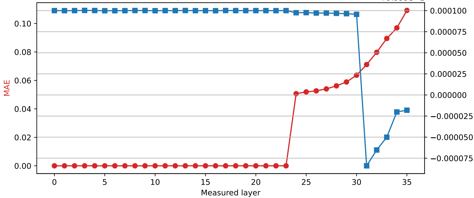
Qwen2.5-3B | Quantized layer 23 | float64 → int8
