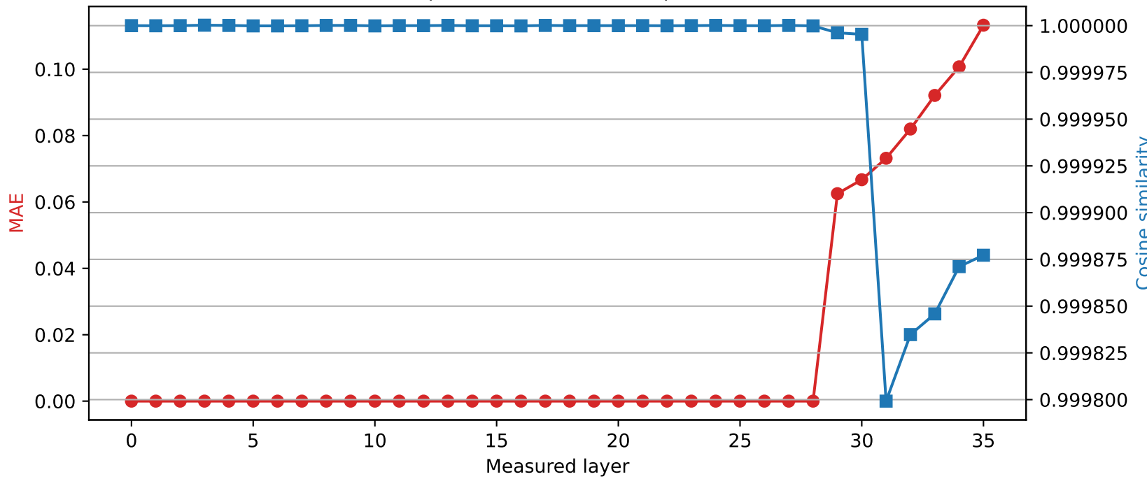
Qwen2.5-3B | Quantized layer 28 | float64 → int8
