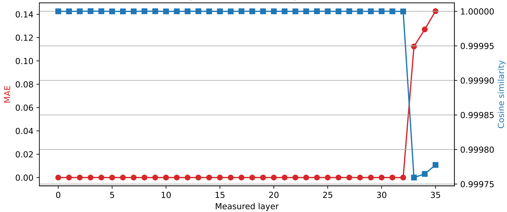
Qwen2.5-3B | Quantized layer 32 | float64 → int8
